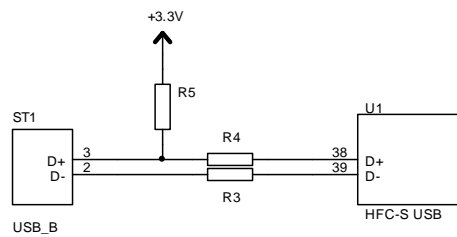
Figure 17: USB connection
