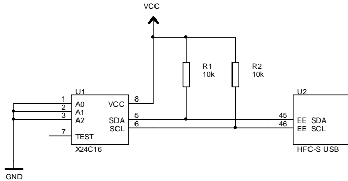
Figure 13: EEPROM circuitry
